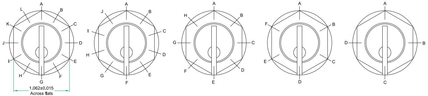
30° INDEXING
