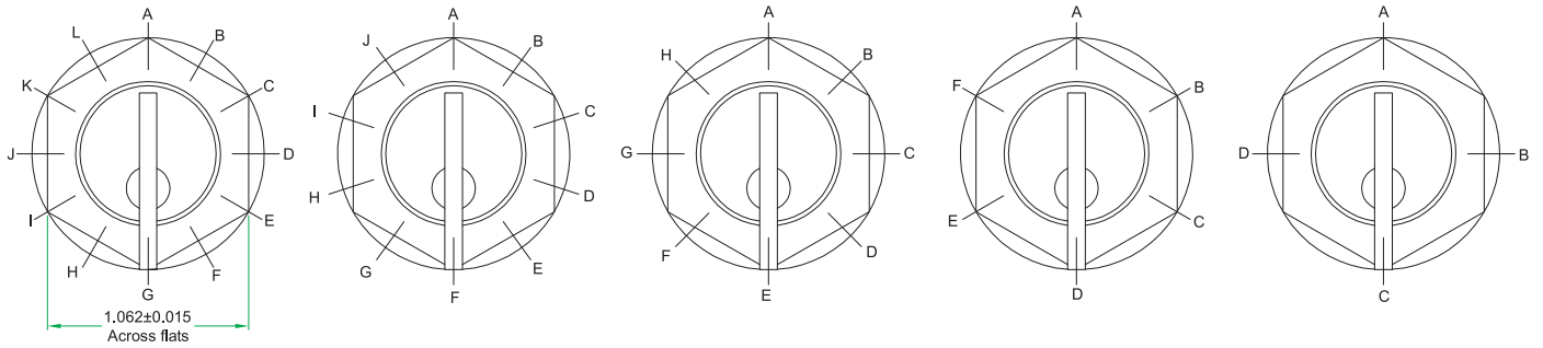
30° INDEXING
